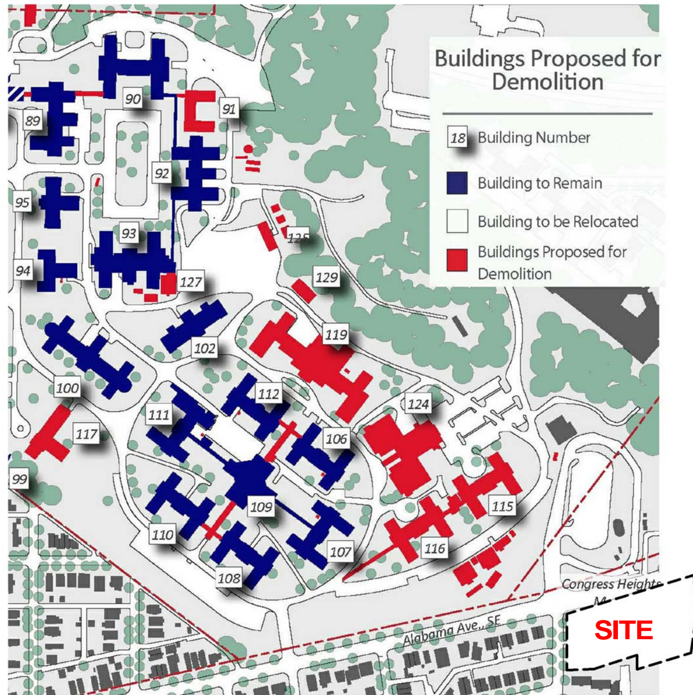
Demolition Plan
